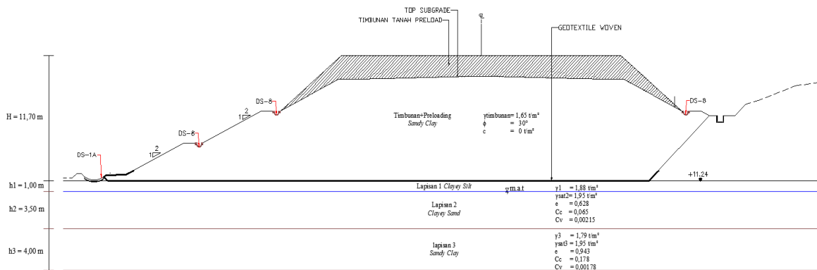
Gambar 9. Gambar asli geometri GeoSlope
