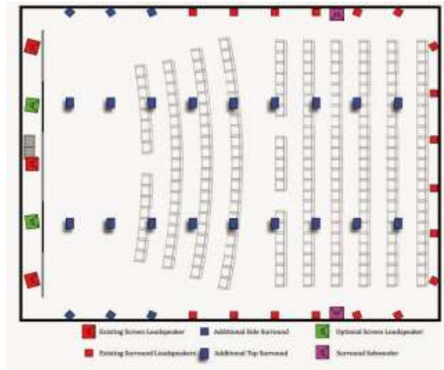
Gambar 1. Skema Instalasi Surround Sound Dolby Atmos
