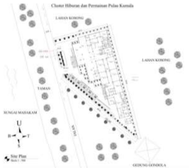
Gambar 9. Site Plan
