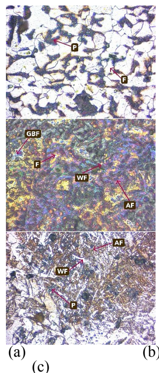
Gambar 5. Struktur Mikro 1,24 KJ/mm (a) Base Metal, (b) HAZ, (c) Weld
